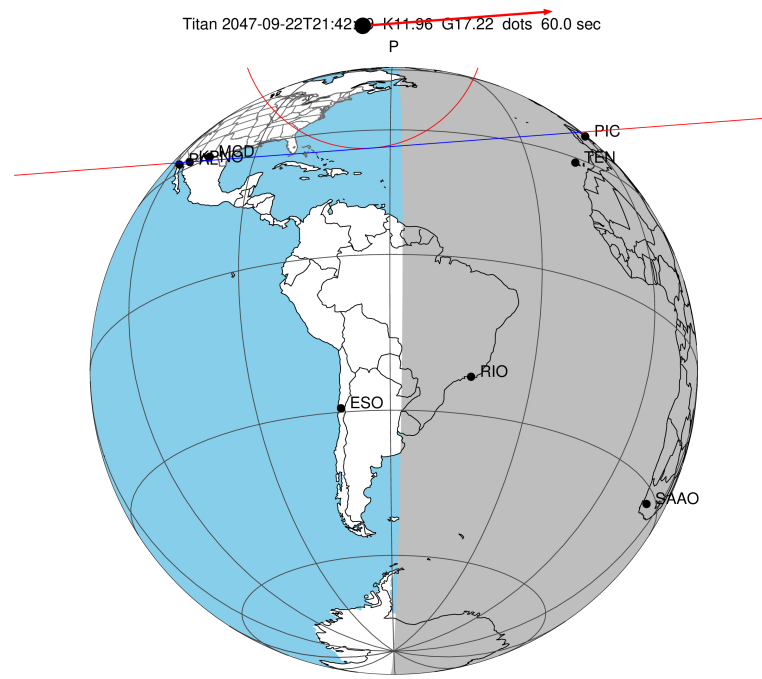
2047-09-22T21:42:49.6600 α: 17 49 46.3431 δ: -22 32 56.389 C/A 1.001" PA 355.65 deg v_sky +12.86 km/s D 10.02 AU Credit: Styled after SORA/Lucky Star
