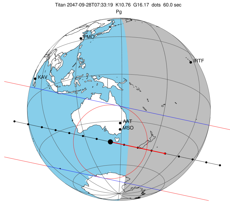
2047-09-28T07:33:19.8100 α: 17 51 01.1879 δ: -22 34 16.872 C/A 0.320" PA 192.10 deg v_sky +16.25 km/s D 10.12 AU Credit: Styled after SORA/Lucky Star
