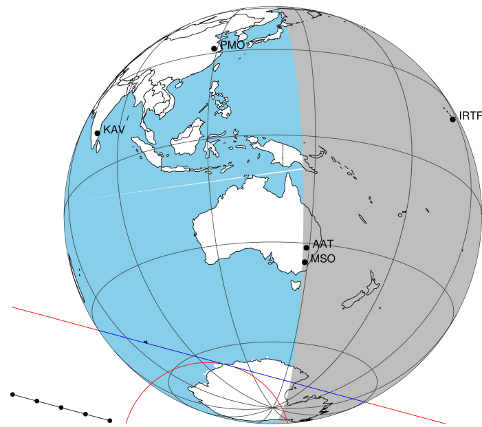
2047-09-30T08:05:17.8500 \alpha : 17 51 25.54 \delta : -22 35 39.825 C/A 1.001" PA 195.07 deg v_sky +12.81 km/s D 10.14 AU Credit: Styled after SORA/Lucky Star
