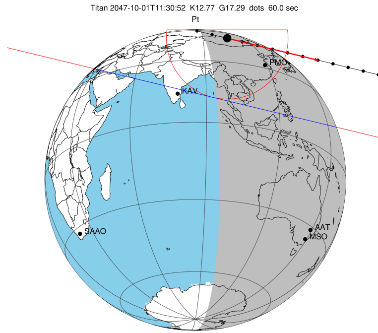
2047-10-01T11:30:52.9500 cc: 17 51 36.6156 d: -22 36 21.697 C/A 0.835" PA 13.58 deg v_sky +10.97 km/s D 10.16 AU Credit: Styled after SORA/Lucky Star
