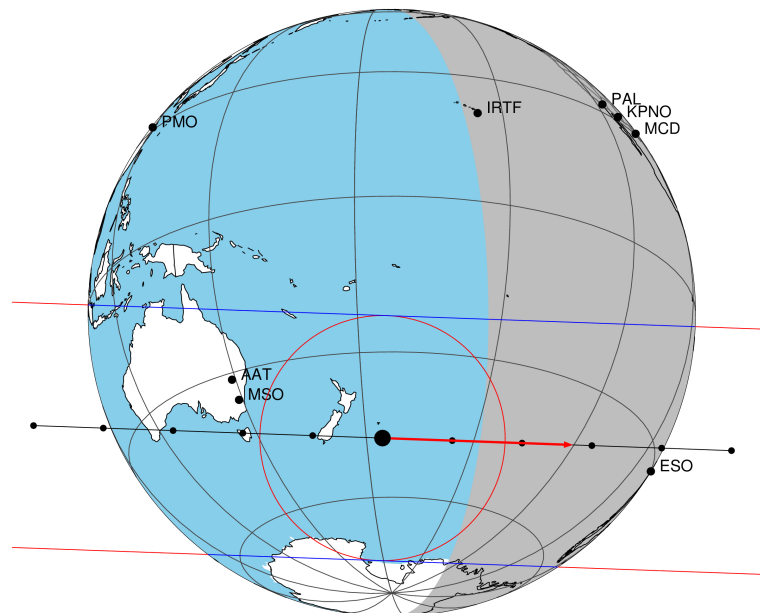
2047-10-11T04:09:31.0800 α: 17 53 41.8670 δ: -22 35 58.617 C/A 0.352" PA 182.06 deg v_sky +24.44 km/s D 10.33 AU Credit: Styled after SORA/Lucky Star
