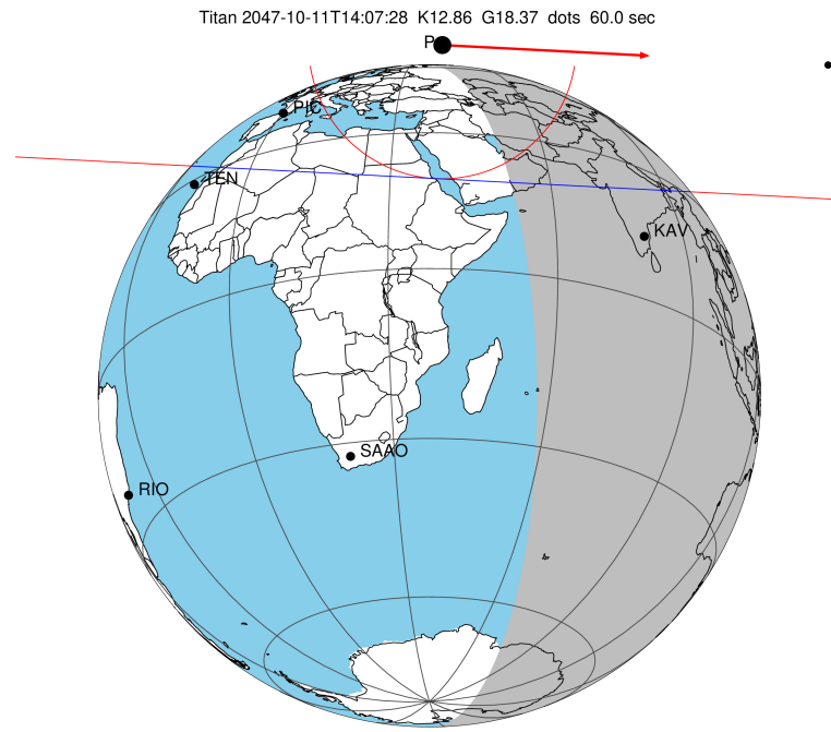
2047-10-11T14:07:28.1000 α: 17 53 50.3704 δ: -22 36 05.033 C/A 0.902" PA 2.96 deg v_sky +24.79 km/s D 10.33 AU Credit: Styled after SORA/Lucky Star
