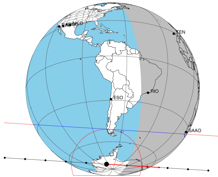
2047-10-11T21:12:54.4400 α: 17 53 56.4841 δ: -22 36 08.242 C/A 0.740" PA 183.59 deg v_sky +24.95 km/s D 10.34 AU Credit: Styled after SORA/Lucky Star
