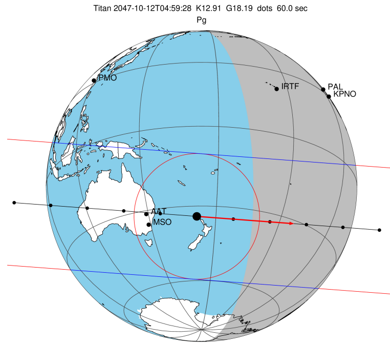
2047-10-12T04:59:28.6200 α: 17 54 03.2060 δ: -22 36 15.237 C/A 0.167" PA 184.26 deg v_sky +25.04 km/s D 10.34 AU Credit: Styled after SORA/Lucky Star
