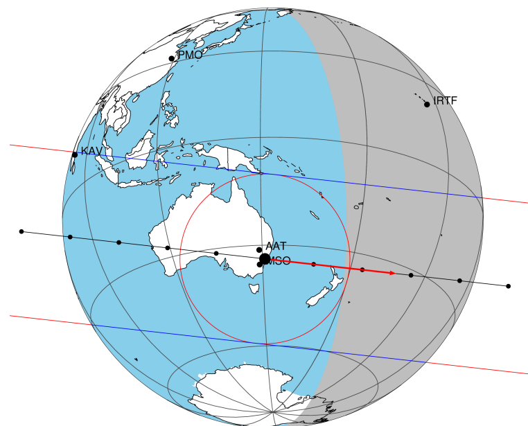
2047-10-13T06:16:33.1800 α: 17 54 24.9764 δ: -22 36 43.571 C/A 0.167" PA 186.42 deg v_sky +24.74 km/s D 10.36 AU Credit: Styled after SORA/Lucky Star
