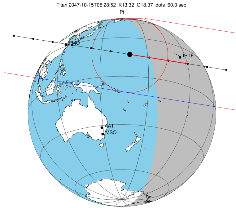
2047-10-15T05:28:52.1100 α: 17 55 03.1065 δ: -22 37 58.029 C/A 0.527" PA 9.17 deg v_sky +22.09 km/s D 10.38 AU Credit: Styled after SORA/Lucky Star
