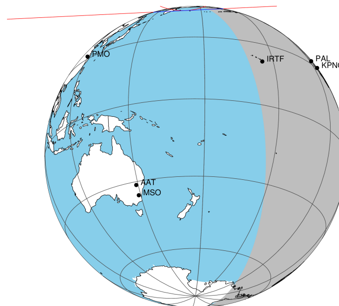
2047-10-21T04:15:27.0600 α: 17 56 33.7315 δ: -22 39 49.889 C/A 1.157" PA 357.21 deg v_sky +19.09 km/s D 10.47 AU
