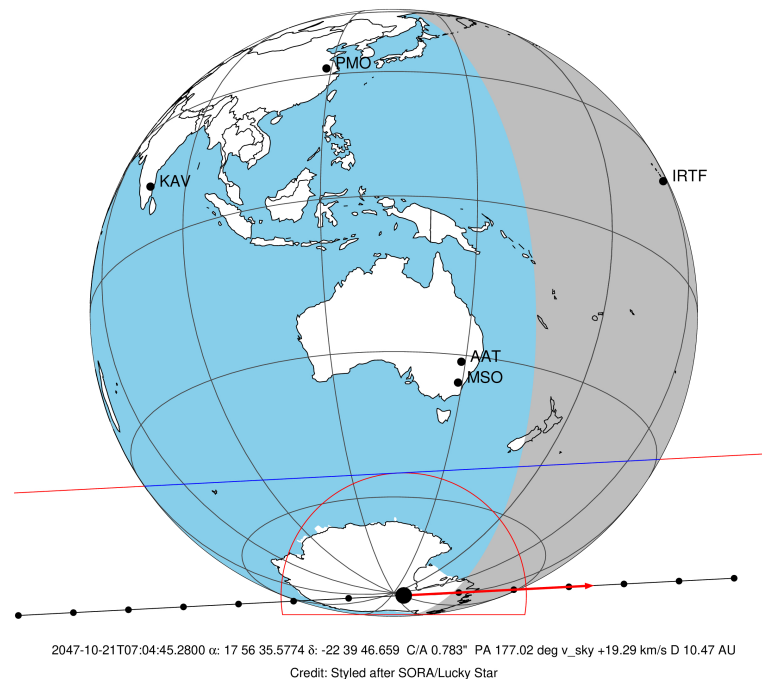
Titan 2047-10-21T07:04:45 K14.31 G18.59 dots 60.0 sec P
