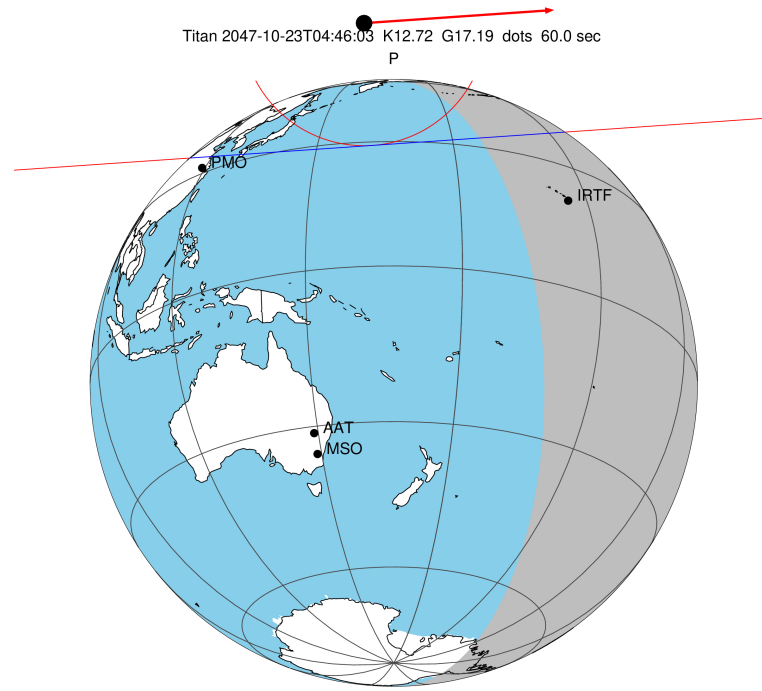
2047-10-23T04:46:03.7200 α: 17 57 08.7866 δ: -22 39 17.880 C/A 0.996" PA 356.04 deg v_sky +23.49 km/s D 10.50 AU Credit: Styled after SORA/Lucky Star
