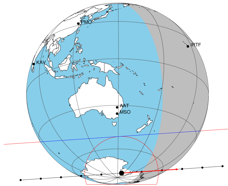
2047-10-23T05:56:04.90000 \alpha : 17 57 09.7145 \delta : -22 39 15.262 C/A 0.732" PA 176.06 deg v_sky +23.61 km/s D 10.50 AU Credit: Styled after SORA/Lucky Star
