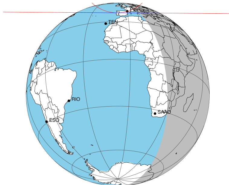
2047-10-26T16:13:00.2600 α: 17 58 26.8005 δ: -22 38 39.384 C/A 1.079" PA 0.38 deg v_sky +30.79 km/s D 10.56 AU
