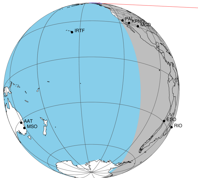
2047-10-28T01:04:07.5000 α: 17 59 01.8329 δ: -22 38 52.614 C/A 1.165" PA 2.71 deg v_sky +31.85 km/s D 10.58 AU
