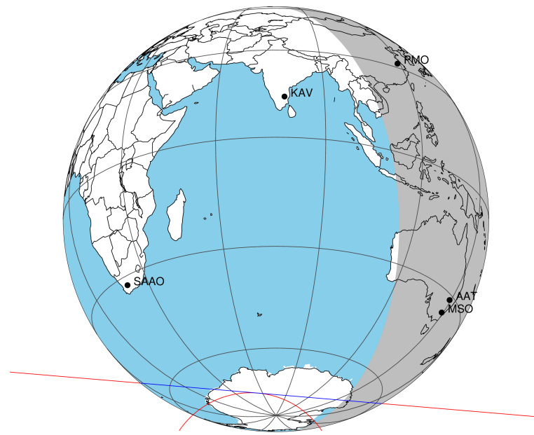
2047-10-29T10:25:45.2400 α: 17 59 37.6098 δ: -22 39 23.386 C/A 1.018" PA 184.85 deg v_sky +31.33 km/s D 10.59 AU Credit: Styled after SORA/Lucky Star
