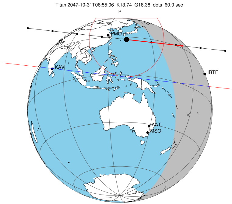
2047-10-31T06:55:06.1000 α: 18 00 22.6260 δ: -22 40 28.796 C/A 0.638" PA 6.55 deg v_sky +28.54 km/s D 10.61 AU Credit: Styled after SORA/Lucky Star
