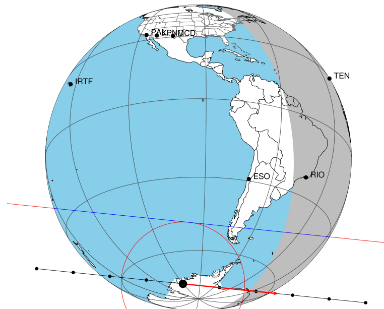
2047-11-01T21:30:54.4400 α: 18 00 57.6019 δ: -22 41 22.0687 PA 185.91 deg v_sky +25.52 km/s D 10.63 AU Credit: Styled after SORA/Lucky Star
