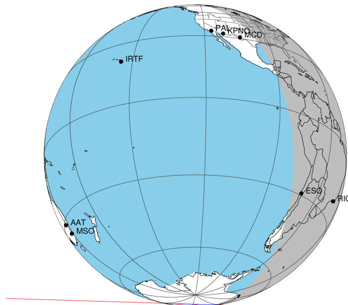
2047-11-03T23:28:07.8200 α: 18 01 38.2753 δ: -22 42 02.017 C/A 1.145" PA 181.77 deg v_sky +23.48 km/s D 10.65 AU Credit: Styled after SORA/Lucky Star
