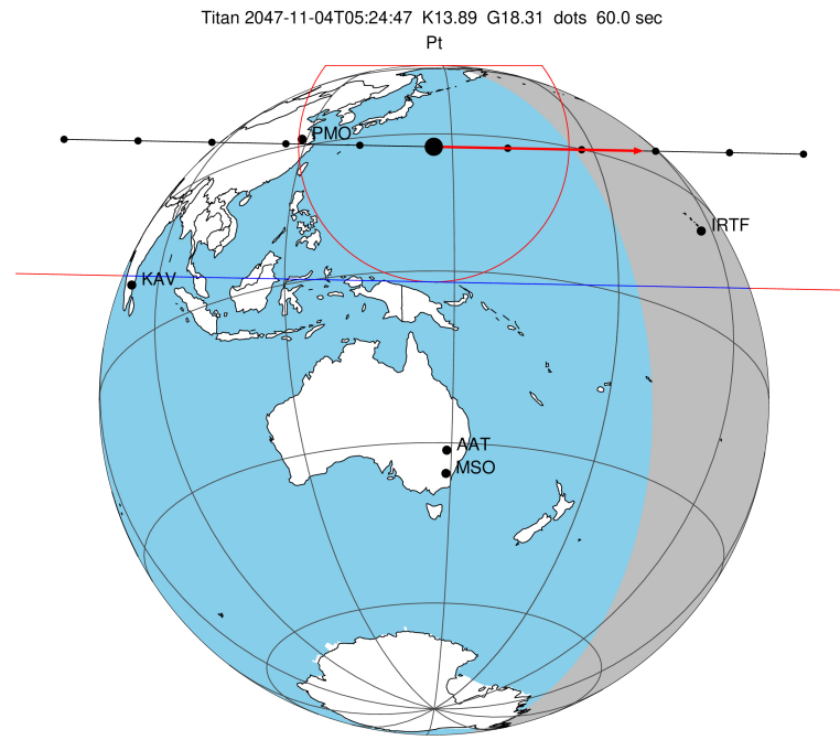
Titan 2047-11-04T05:24:47 K13.89 G18.31 dots 60.0 sec 2047-11-04T05:24:47.6800 α: 18 01 42.96811 δ: -22 42 05.438 C/A 0.624" PA 1.15 deg v_sky +23.48 km/s D 10.66 AU Credit: Styled after SORA/Lucky Star
