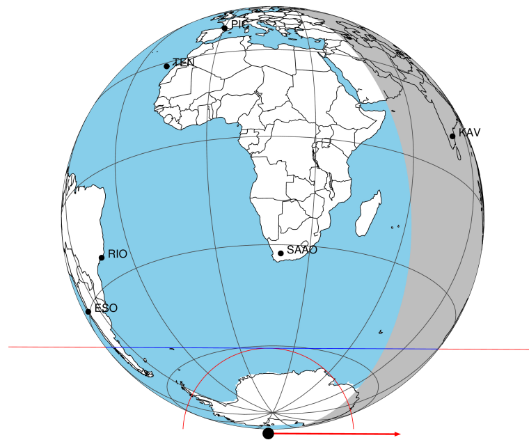
2047-11-04T13:56:44.5500 \alpha : 18 01 49.7213 \delta : -22 42 05.127 C/A 0.842" PA 180.27 deg v_sky +23.57 km/s D 10.66 AU Credit: Styled after SORA/Lucky Star
