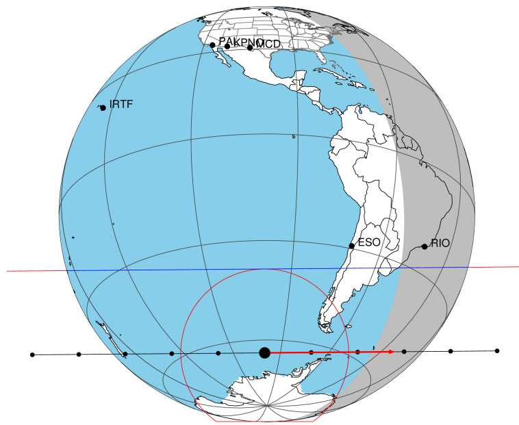
2047-11-04T21:42:52.8700 α: 18 01 55.9032 δ: -22 42 05.256 C/A 0.551" PA 179.52 deg v_sky +23.75 km/s D 10.66 AU Credit: Styled after SORA/Lucky Star
