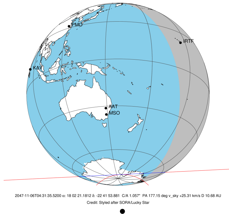
Titan 2047-11-06T04:31:35 K13.13 G18.02 dots 60.0 sec P
