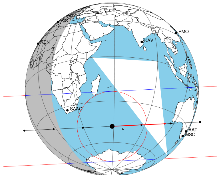
2048-02-17T05:13:58.8900 α: 18 51 26.2051 δ: -22 15 43.849 C/A 0.350" PA 177.22 deg v_sky +35.93 km/s D 10.72 AU Credit: Styled after SORA/Lucky Star
