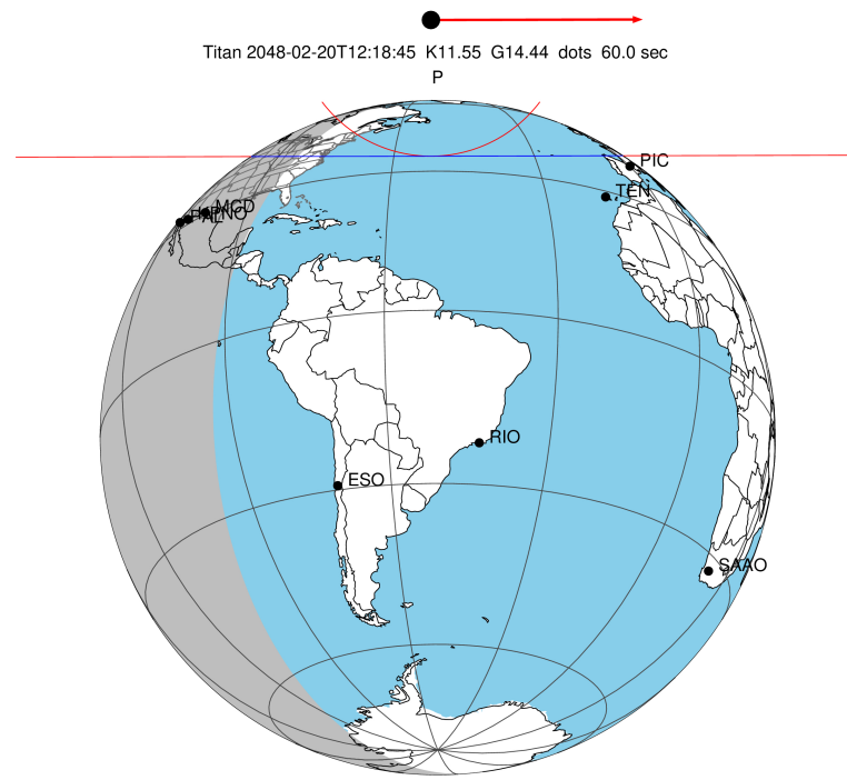
2048-02-20T12:18:45.8000 α: 18 52 54.8038 δ: -22 15 22.200 C/A 1.021" PA 359.86 deg v_sky +29.92 km/s D 10.67 AU Credit: Styled after SORA/Lucky Star
