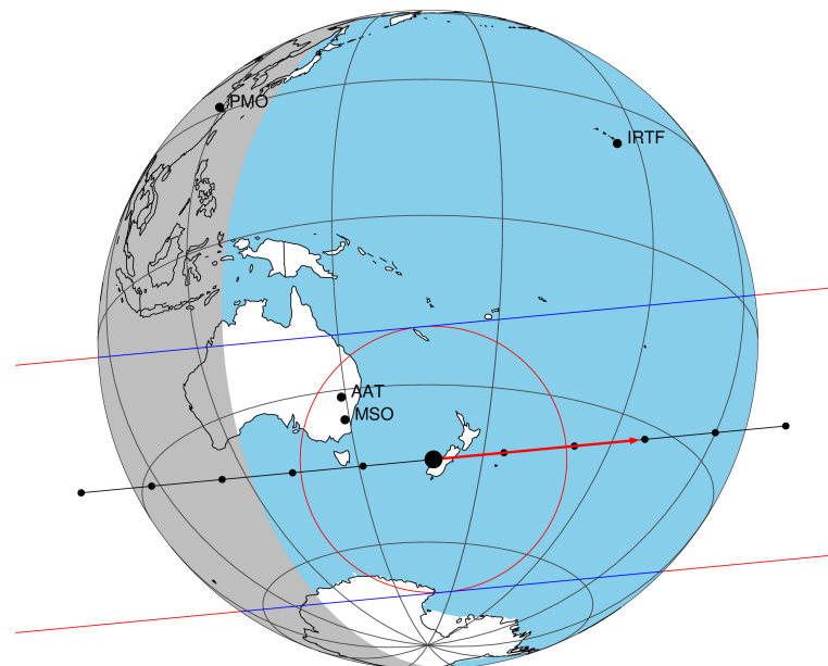
2048-02-23T21:35:15.1100 α: 18 54 05.3458 δ: -22 14 48.014 C/A 0.300" PA 174.58 deg v_sky +22.79 km/s D 10.62 AU Credit: Styled after SORA/Lucky Star
