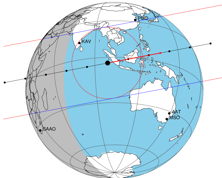
2048-02-28T01:36:43.0600 α: 18 55 22.1028 δ: -22 11 53.284 C/A 0.267" PA 349.21 deg v_sky +25.10 km/s D 10.57 AU Credit: Styled after SORA/Lucky Star
