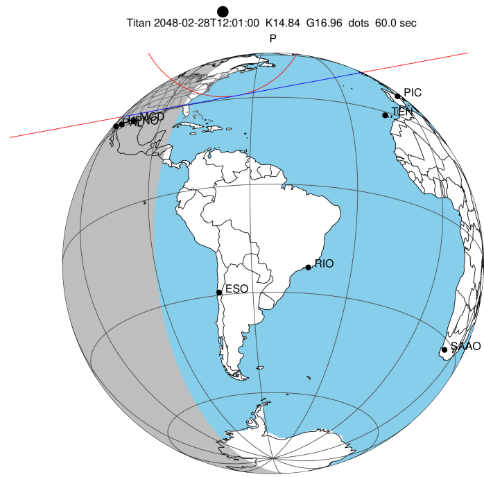
2048-02-28T12:01:00.1600 α: 18 55 30.9150 δ: -22 11 31.073 C/A 1.015" PA 349.54 deg v_sky +25.78 km/s D 10.56 AU Credit: Styled after SORA/Lucky Star
