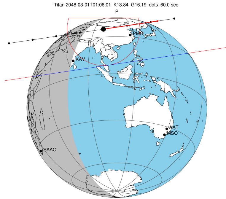
2048-03-01T01:06:01.5300 α: 18 56 04.3471 δ: -22 10 12.434 C/A 0.737" PA 351.48 deg v_sky +28.17 km/s D 10.54 AU Credit: Styled after SORA/Lucky Star
