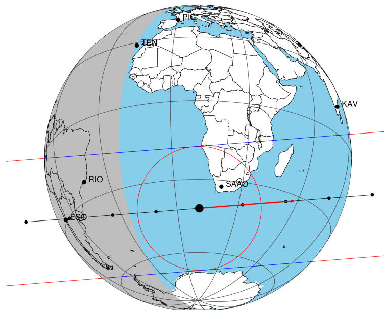
2048-03-03T07:31:18.6300 α: 18 56 58.1961 δ: -22 08 45.632 C/A 0.273" PA 175.48 deg v_sky +30.07 km/s D 10.51 AU Credit: Styled after SORA/Lucky Star
