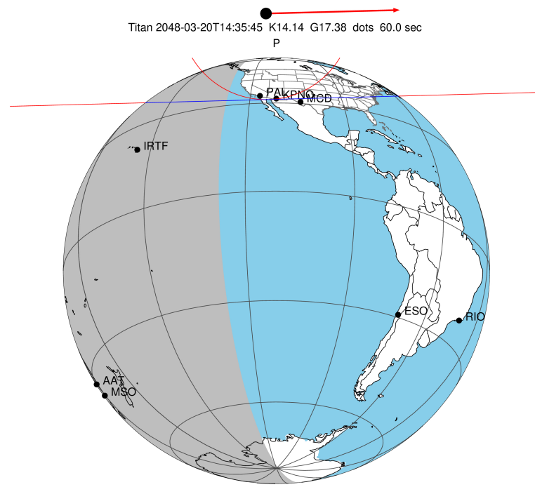
2048-03-20T14:35:45.6100 α: 19 02 01.4366 δ: -22 02 09.515 C/A 1.037" PA 358.49 deg v_sky +22.31 km/s D 10.25 AU Credit: Styled after SORA/Lucky Star
