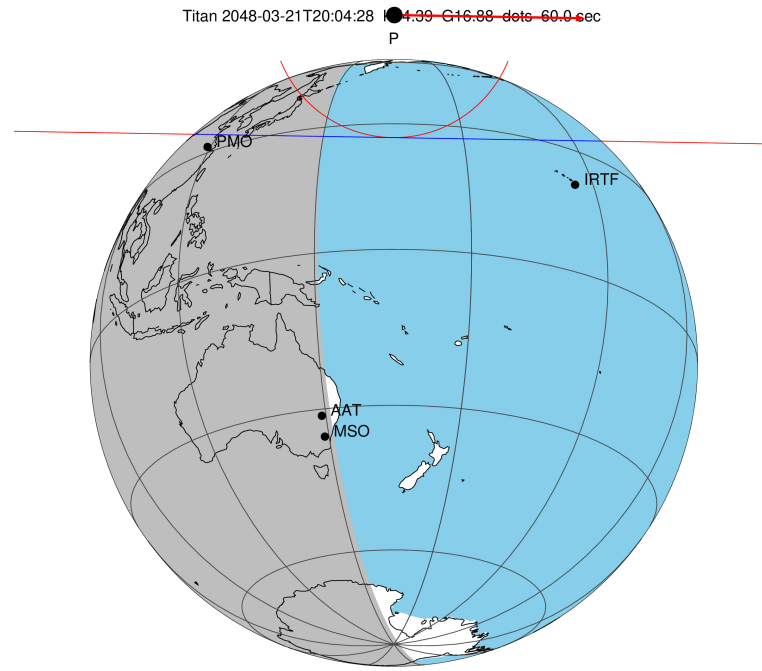
2048-03-21T20:04:28.2200 α: 19 02 23.4928 δ: -22 02 08.146 C/A 0.985" PA 0.96 deg v_sky +20.41 km/s D 10.23 AU Credit: Styled after SORA/Lucky Star
