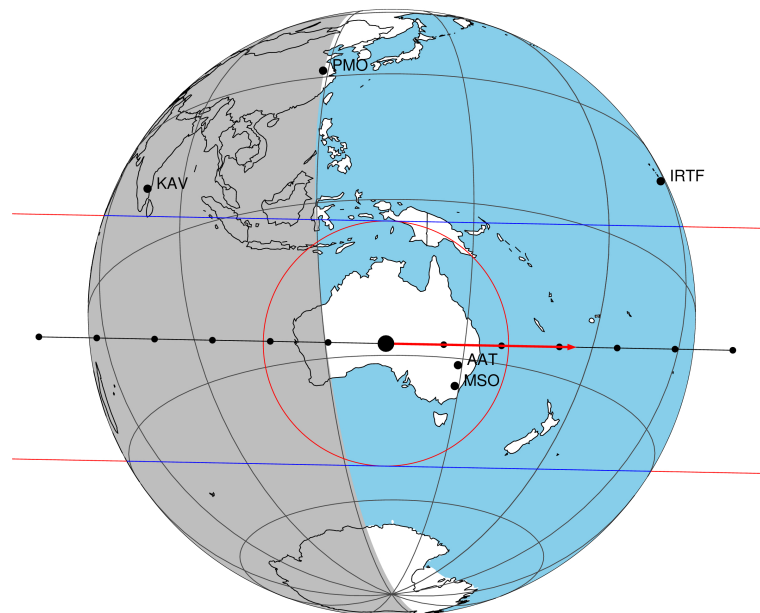
2048-03-21T22:07:34.0300 α: 19 02 24.9497 δ: -22 02 07.439 C/A 0.087" PA 181.06 deg v_sky +20.24 km/s D 10.23 AU Credit: Styled after SORA/Lucky Star
