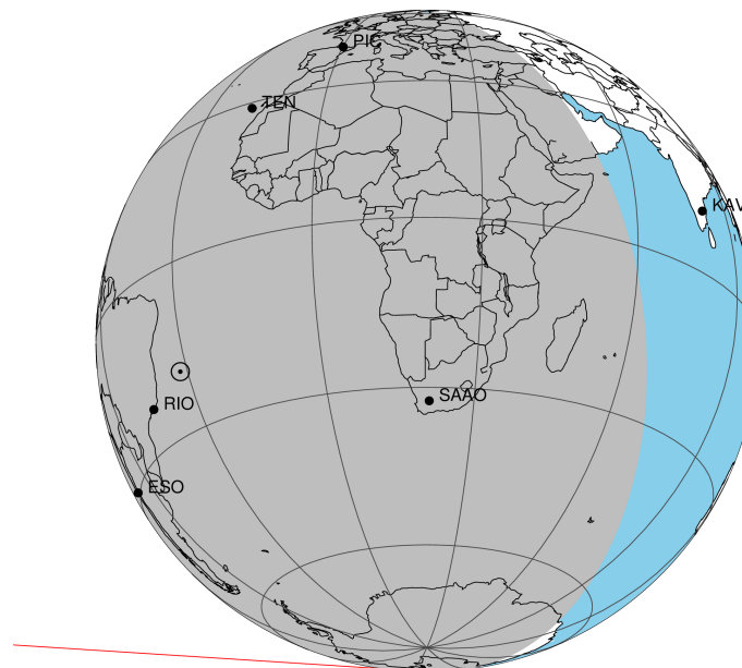
2048-05-17T02:03:48.1900 cc: 19 04 11.4339 s -22 01 10.348 C/A 1.320" PA 183.68 deg v_sky -13.14 km/s D 09.34 AU
