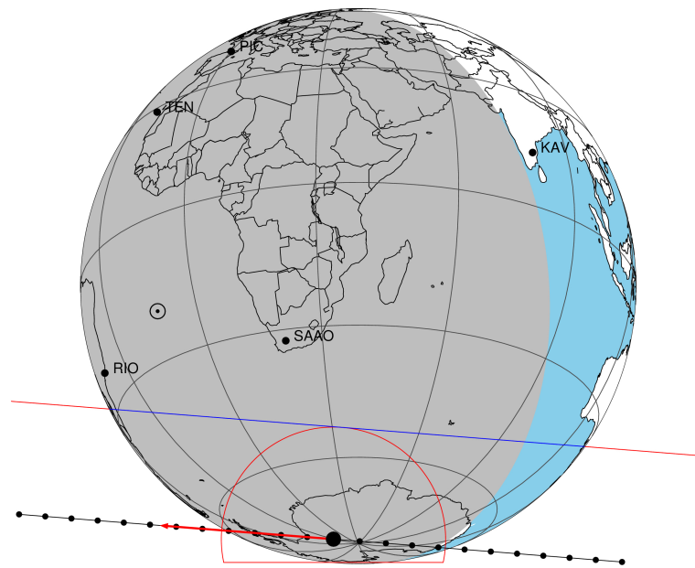
2048-05-19T00:41:51.9000 cc: 19 03 50.6783 & -22 00 47.999 C/A 0.864" PA 184.52 deg v_sky -10.06 km/s D 09.32 AU Credit: Styled after SORA/Lucky Star
