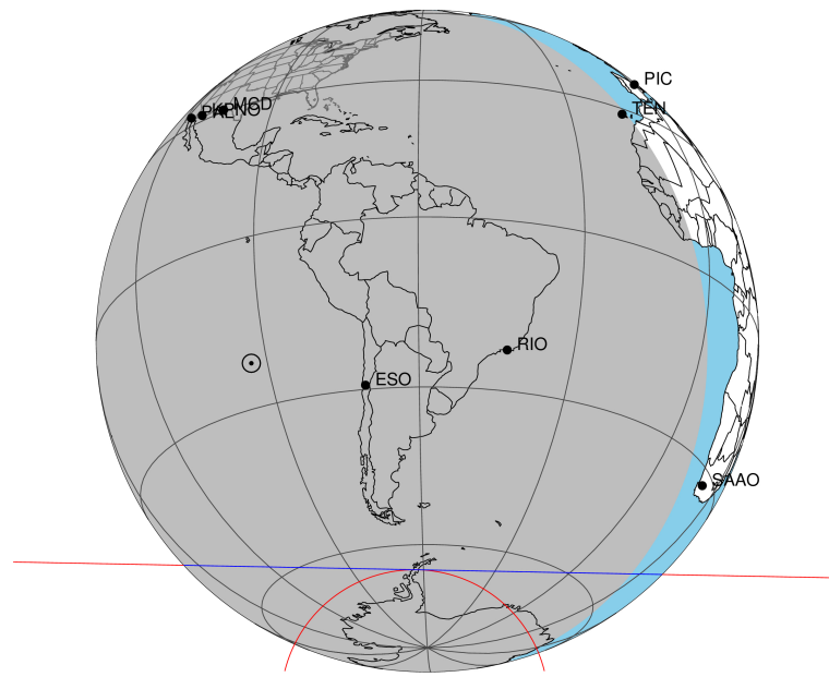
2048-06-02T06:11:42.2300 cc: 19 00 58.1007 & -22 06 34.235 C/A 1.051" PA 181.10 deg v_sky -18.07 km/s D 09.16 AU Credit: Styled after SORA/Lucky Star
