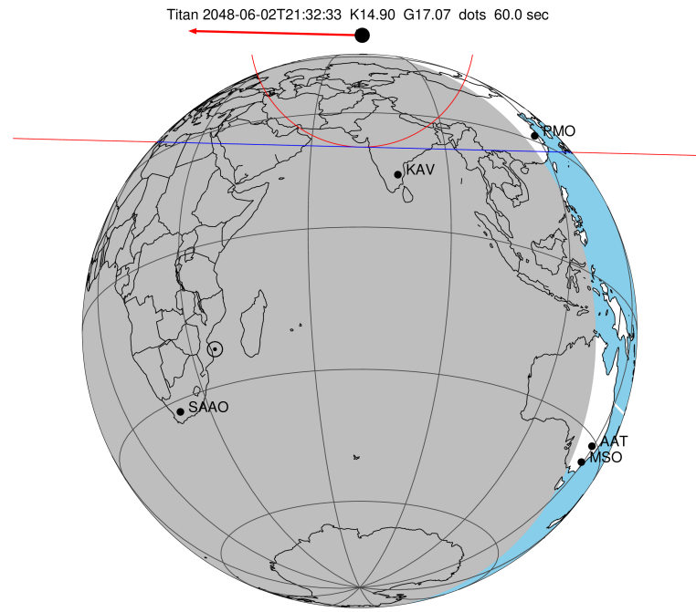
2048-06-02T21:32:33.7900 α: 19 00 47.5942 δ: -22 06 33.007 C/A 1.025" PA 1.43 deg v_sky -17.03 km/s D 09.16 AU Credit: Styled after SORA/Lucky Star
