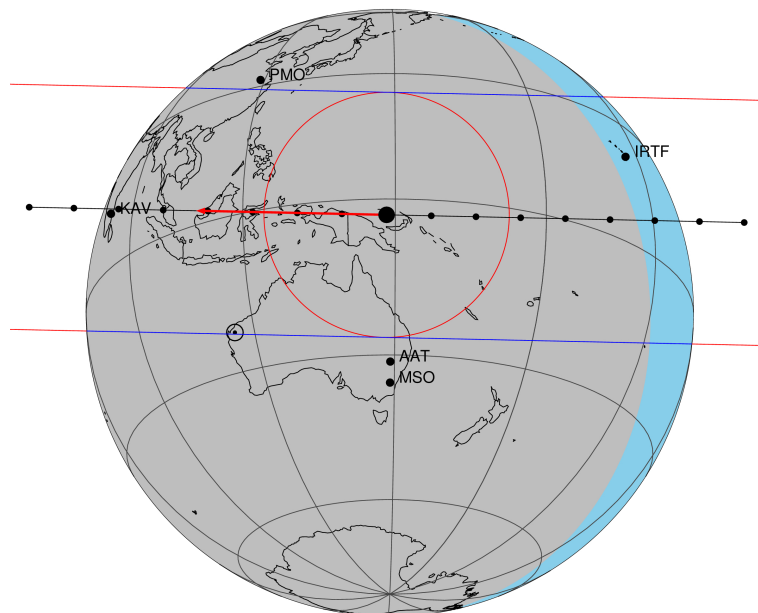
2048-06-03T16:16:21.1200 α: 19 00 35.6618 δ: -22 06 28.267 C/A 0.310" PA 1.23 deg v_sky -15.64 km/s D 09.15 AU Credit: Styled after SORA/Lucky Star
