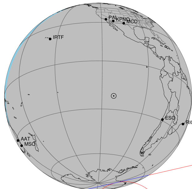
2048-07-13T07:34:44.6400 cc: 18 49 11.4375 s: -22 25 34.919 PA 1.309" PA 167.06 deg v_sky -20.21 km/s D 09.03 AU Credit: Styled after SORA/Lucky Star
