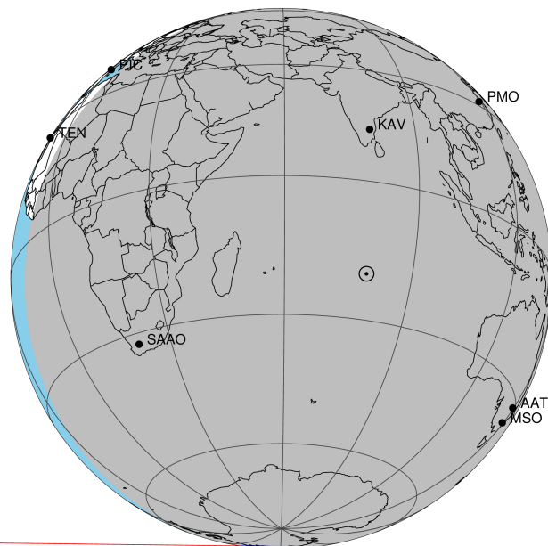
2048-07-21T18:50:54.3500 cc: 18 46 10.9492 d: -22 28 31.539 C/A 1.352" PA 180.68 deg v_sky -17.47 km/s D 09.07 AU Credit: Styled after SORA/Lucky Star
