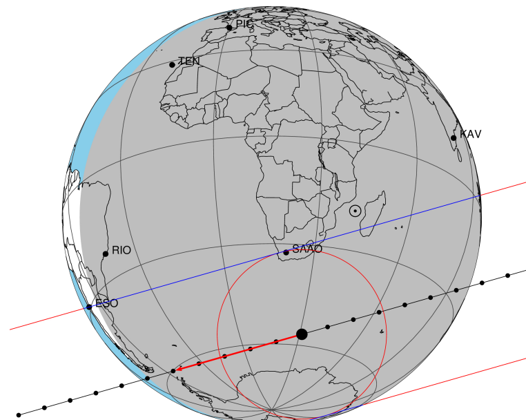
2048-07-26T21:22:11.0900 α: 18 45 04.5013 δ: -22 30 19.142 C/A 0.562" PA 164.07 deg v sky -13.57 km/s D 09.10 AU
