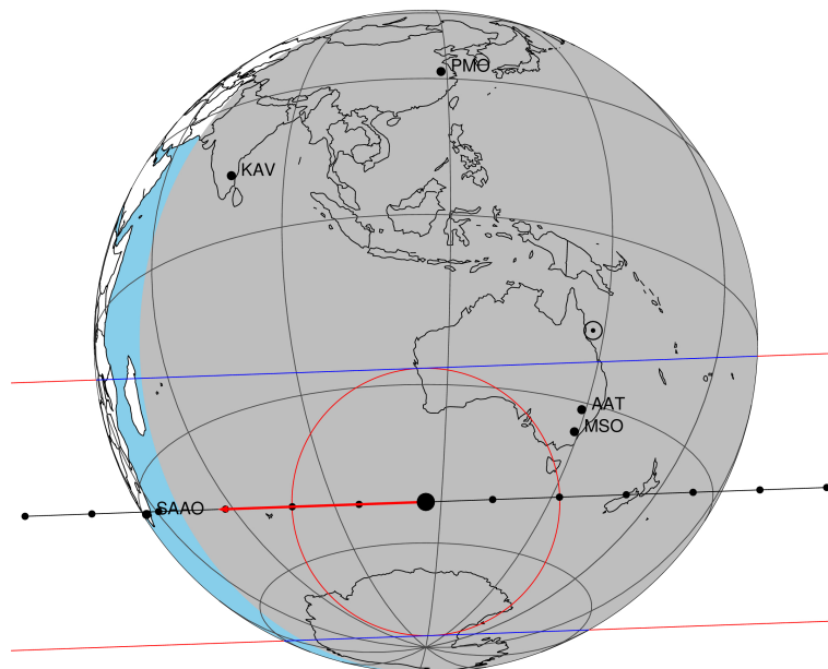
2048-08-02T14:15:38.4800 cc: 18 43 07.6477 & -22 35 03.331 C/A 0.466" PA 177.93 deg v_sky -21.41 km/s D 09.14 AU Credit: Styled after SORA/Lucky Star
