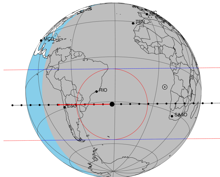
2048-08-07T23:40:36.56000 cc: 18 41 42.8790 s -22 34 41.881 C/A 0.151" PA 179.40 deg v_sky -10.96 km/s D 09.20 AU Credit: Styled after SORA/Lucky Star
