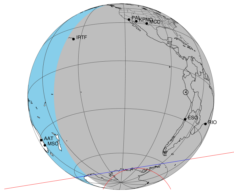
2048-08-16T05:13:03.3000 cc: 18 40 20.67033 s -22 39 30.872 C/A 1.124" PA 170.85 deg v_sky -16.19 km/s D 09.28 AU Credit: Styled after SORAV Sky Star
