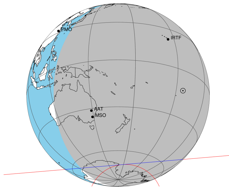
2048-08-17T09:40:58.4000 cc: 18 40 02.6081 & -22 40 01.423 C/A 1.103" PA 175.13 deg v_sky -16.74 km/s D 09.29 AU
