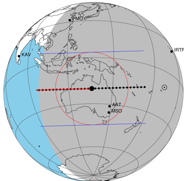
2048-08-24T11:20:09.2700 α: 18 38 47.0107 δ: -22 39 23.809 C/A 0.037" PA 358.31 deg v_sky - 4.16 km/s D 09.39 AU Credit: Styled after SORA/Lucky Star
