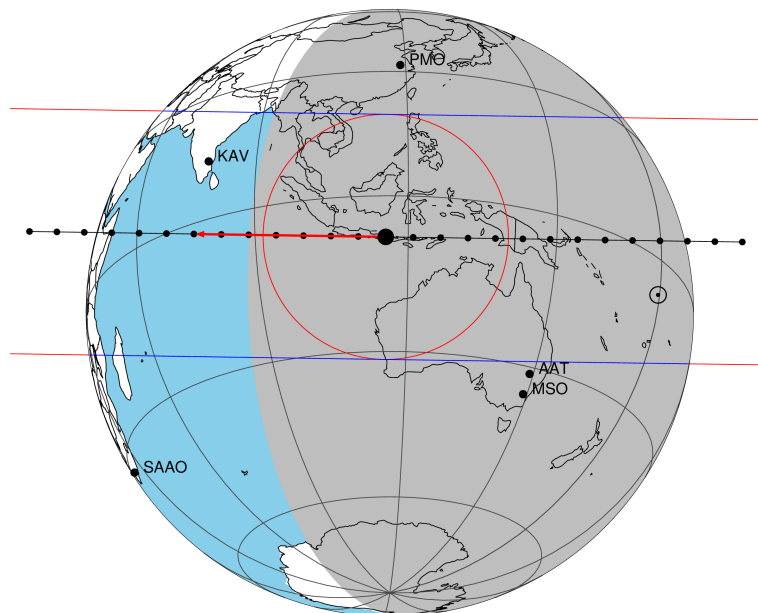
2048-09-03T12:01:33.5500 α: 18 37 53.1823 δ: -22 43 53.981 C/A 0.231" PA 0.84 deg v_sky - 9.60 km/s D 09.52 AU
