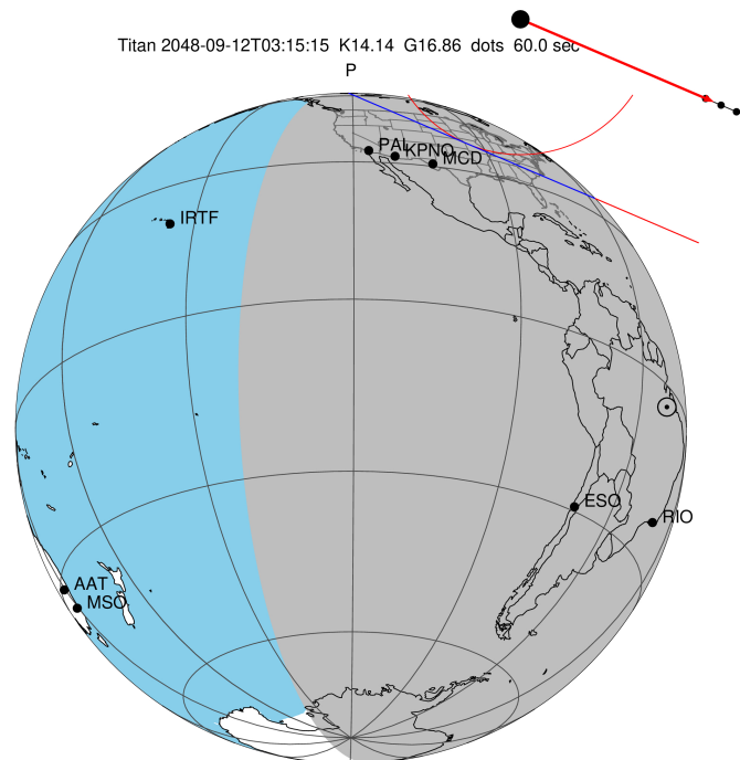
2048-09-12T03:15:15.6700 α: 18 37 43.6657 δ: -22 43 00.757 C/A 1.202" PA 23.15 deg v_sky + 5.32 km/s D 09.66 AU Credit: Styled after SORA/Lucky Star
