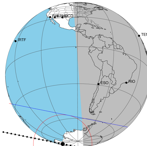
2048-10-02T23:51:09.540000 cc: 18 39 14.8636 d: -22 46 12.728 C/A 0.865" PA 191.32 deg v_sky + 5.90 km/s D 09.99 AU Credit: Styled after SORA/Lucky Star
